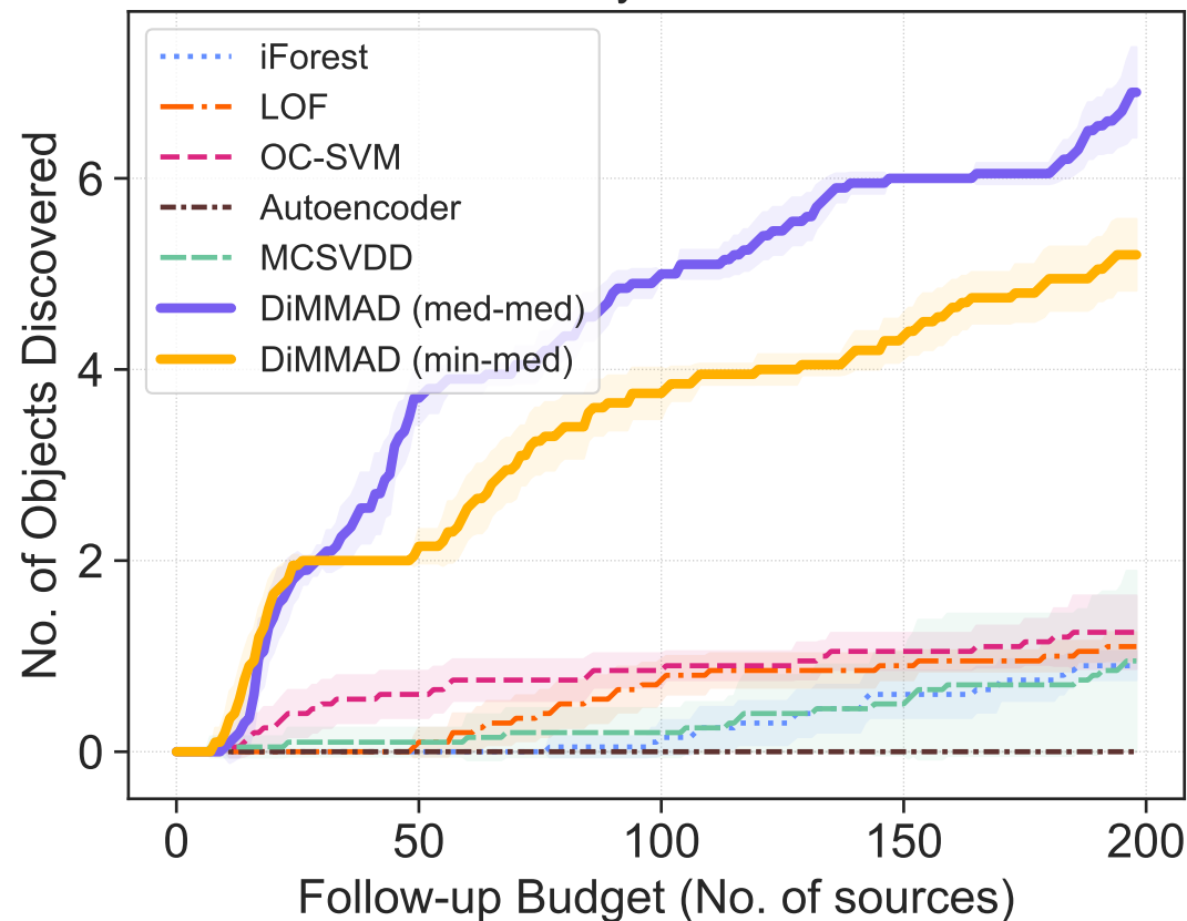
Anomaly: SL-SN1a
